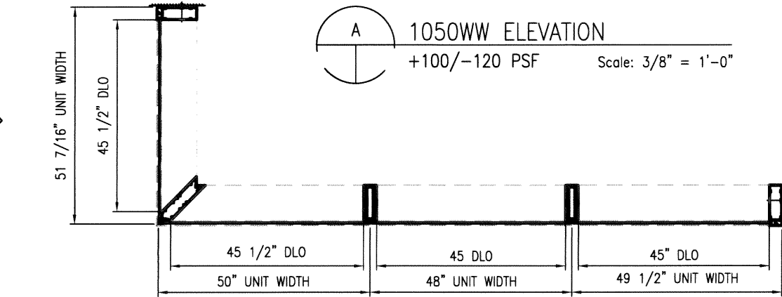
PLAN 1050WW PLAN +100/-120 PSF Scale: 3/8" = 1'-0"
