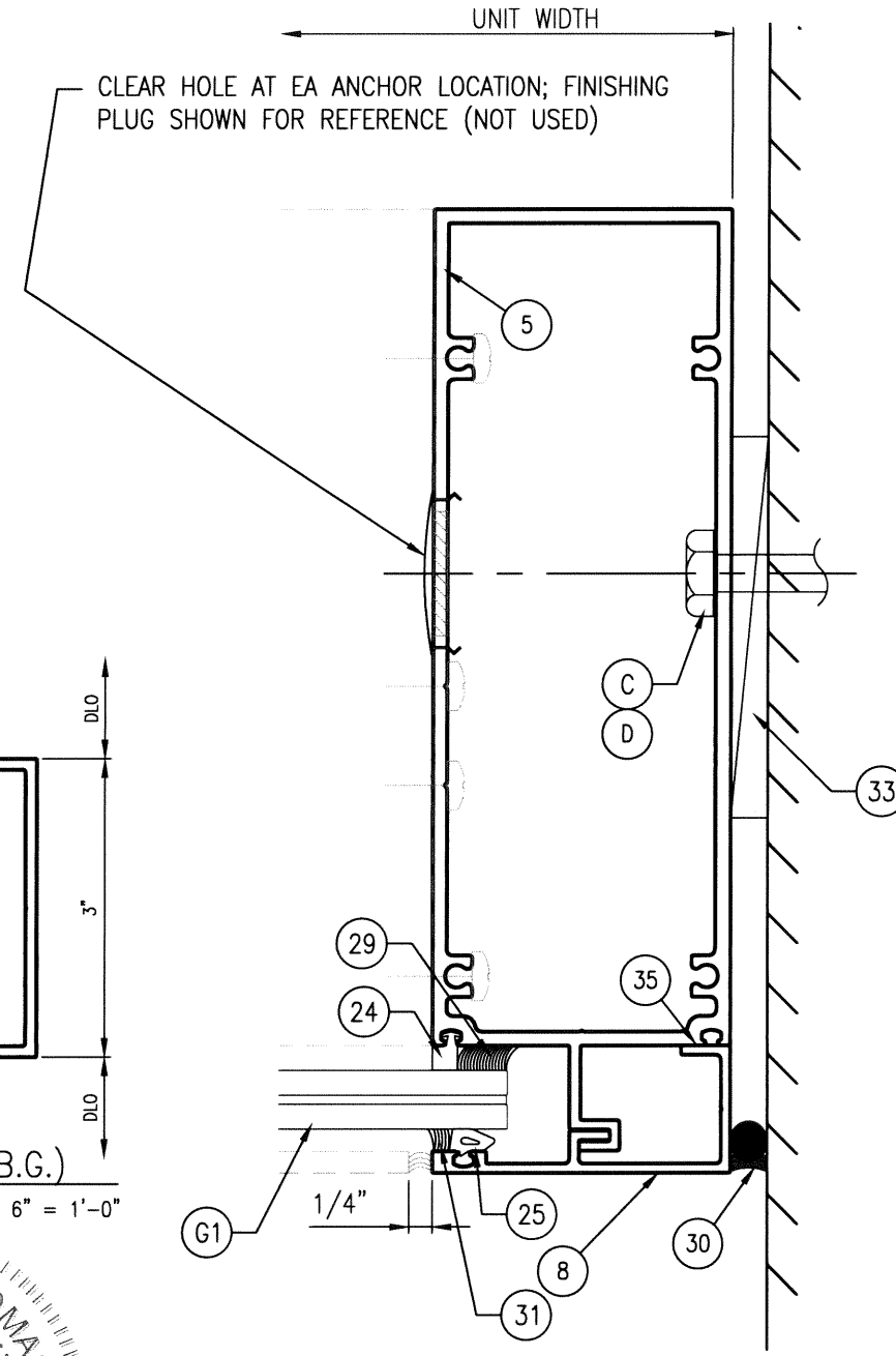
4 ANCHORED JAMB Glazing condition G1 Scale: 6" = 1'-0"
