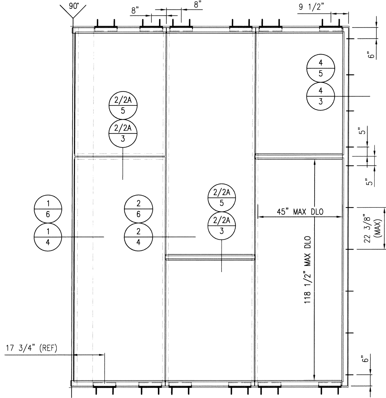
A 1050WW ELEVATION +100/-120 PSF Scale: 3/8" = 1'-0"
