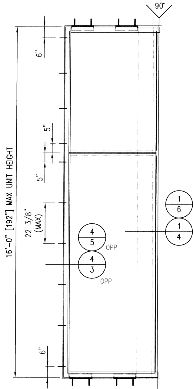
B 1050WW ELEVATION +100/-120 PSF Scale: 3/8" = 1'-0"
