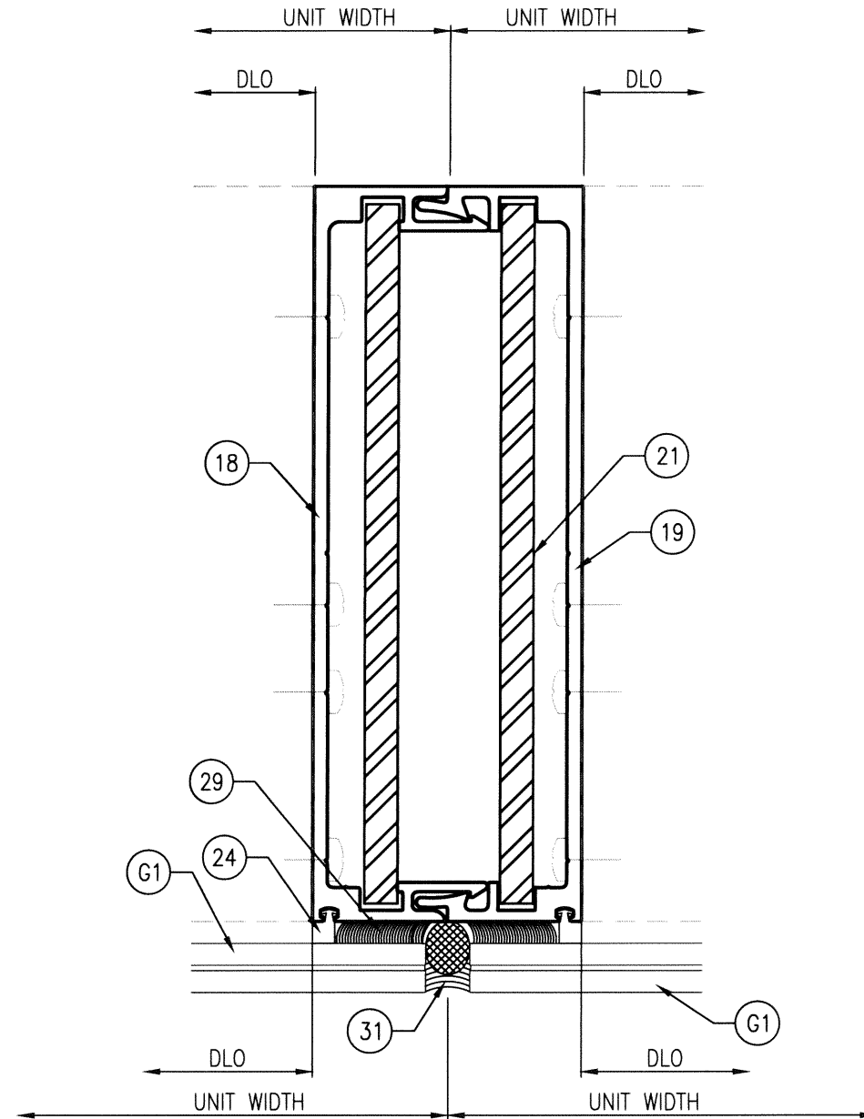
2 REINFORCED MULLION 1050WW Scale: 6" = 1'-0"
